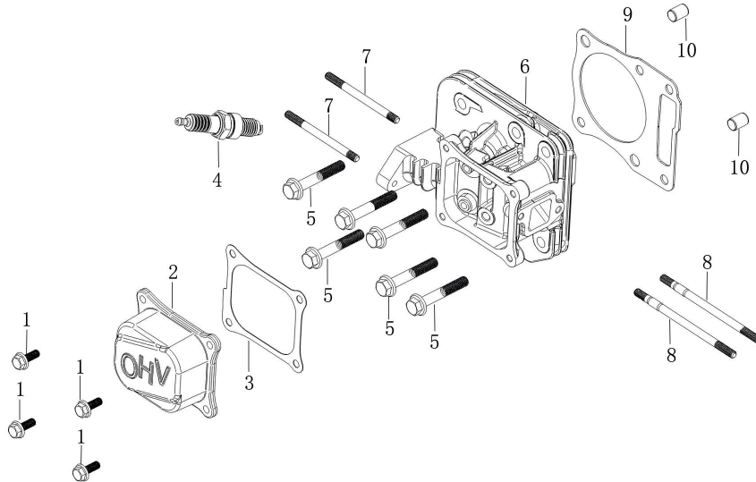
RYS A - CYLINDER HEAD
