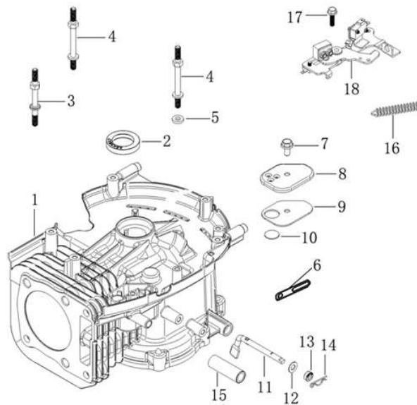
RYS B - CRANK CASE
