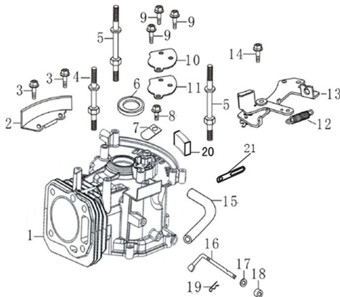
RYS B - CRANK CASE
