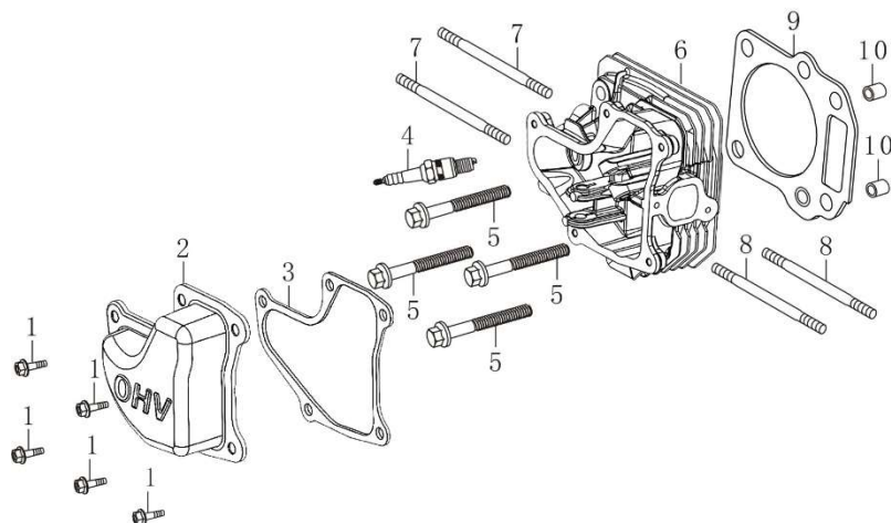
RYS A - CYLINDER HEAD
